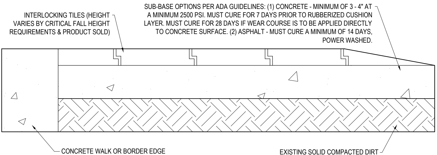
SECTION VIEW
