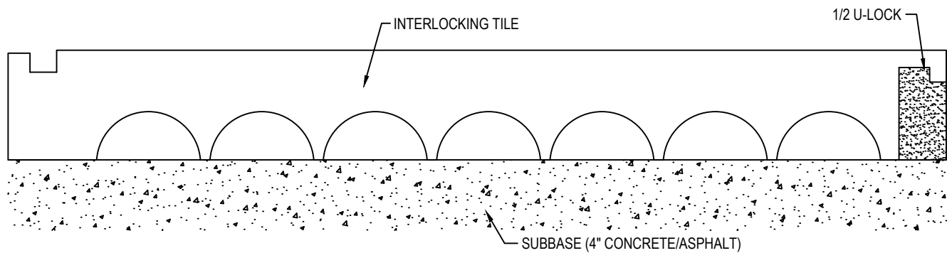
SECTION VIEW FEMALE LOCK WITH 1/2 U-LOCK (WHEN USE WITH CONCRETE CURB)
