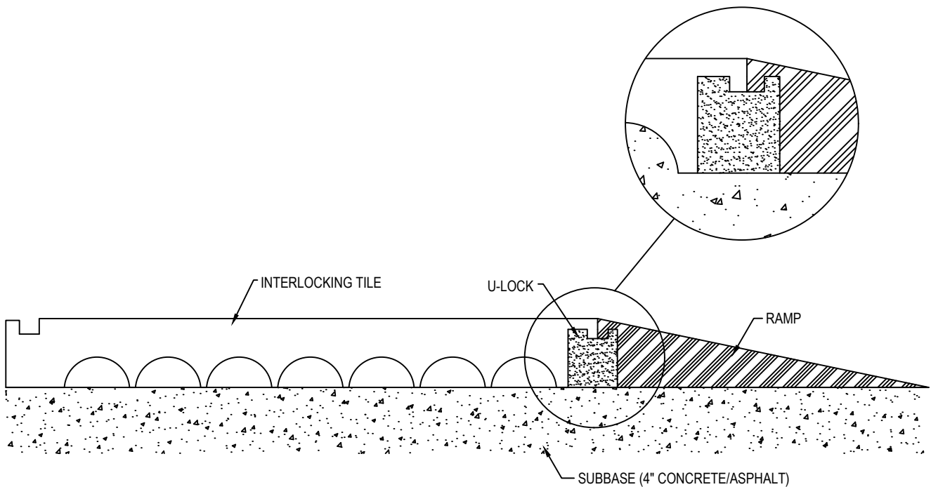
SECTION VIEW FEMALE LOCK WITH 1/2 U-LOCK (WHEN USE WITH CONCRETE CURB)
