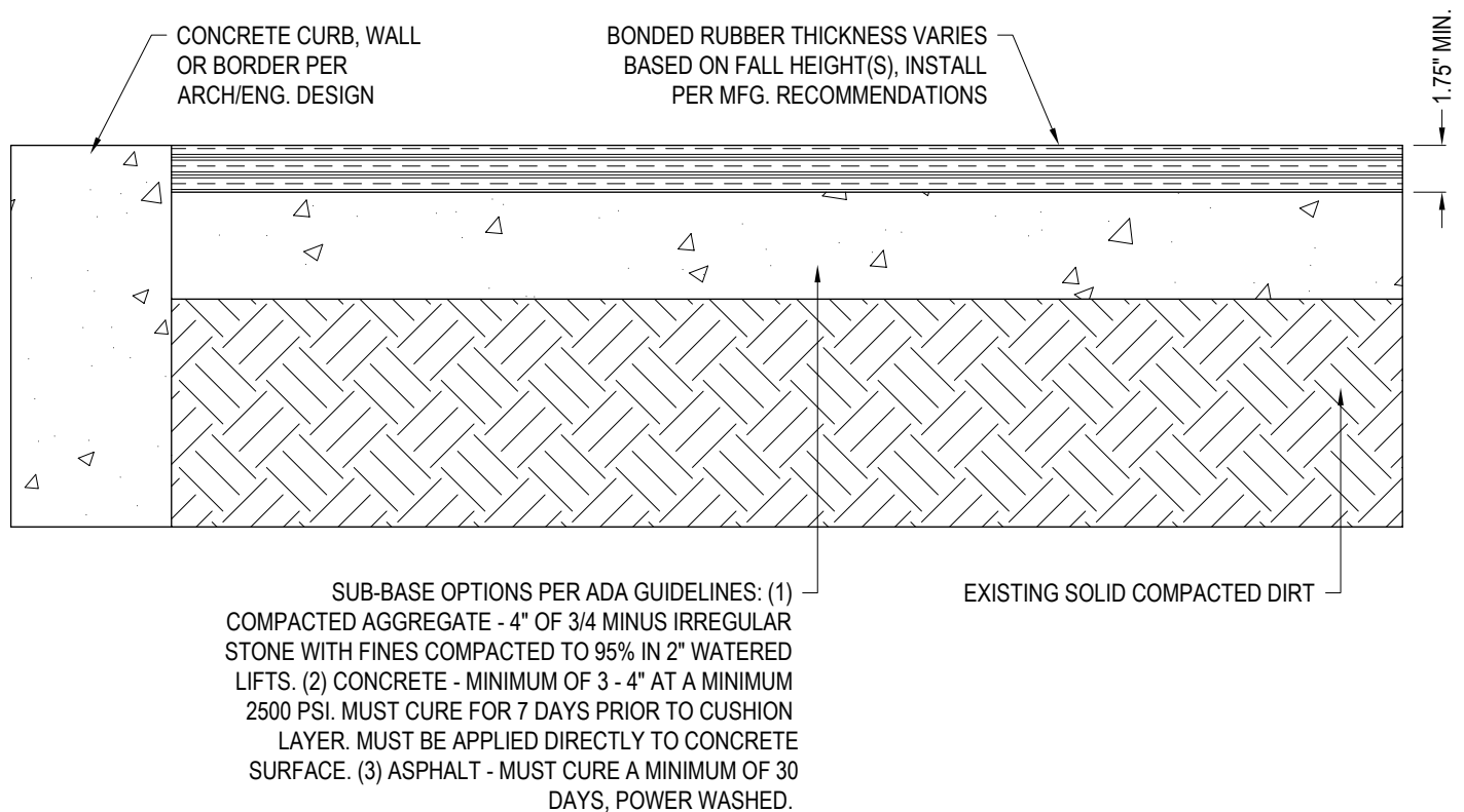
SECTION VIEW
